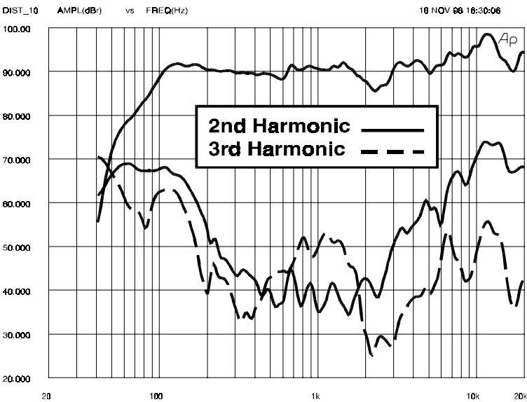
Figure 5—Sx80T Harmonic Distortion Response 10% Rated Power Input (17.5 watts), (full-space anechoic environment, 3.05 meters (10 feet) on axis)
